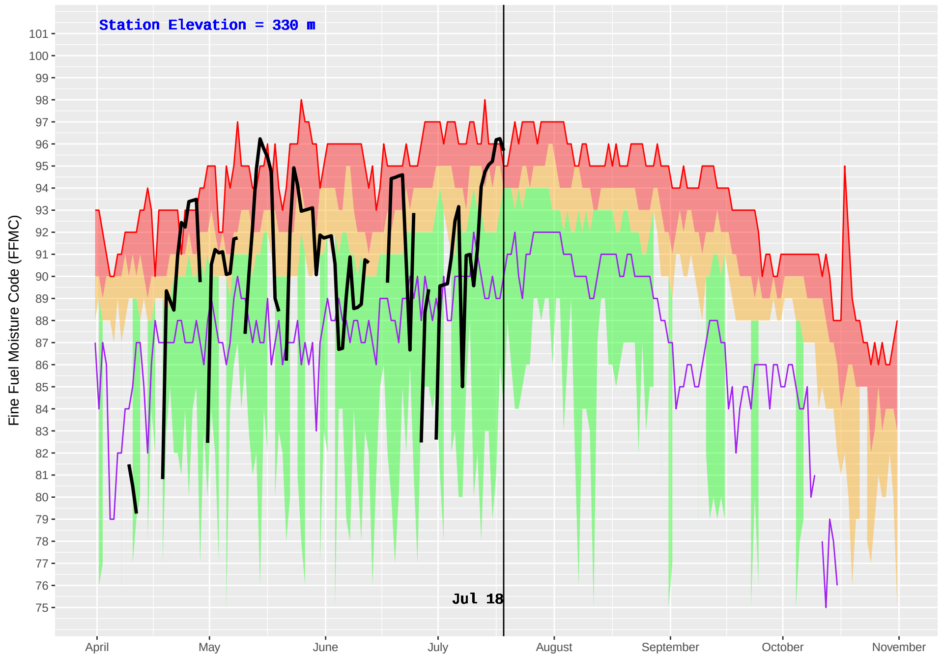
D'ARCY (292) : Historical (1978–2016) and Current (2018) Daily Fine Fuel Moisture Code (FFMC)
