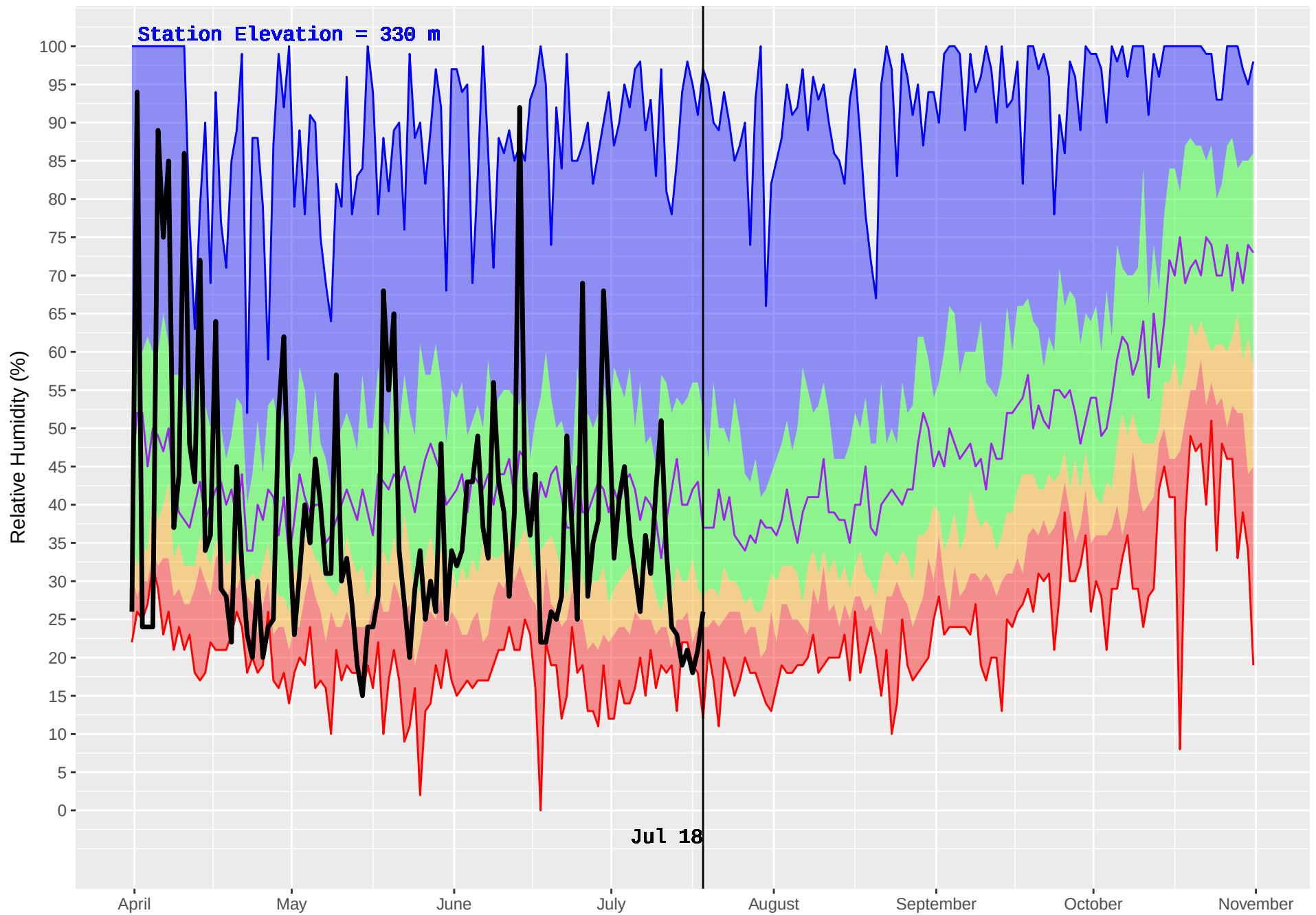
D'ARCY (292) : Historical (1978–2016) and Current (2018) Daily Relative Humidity
